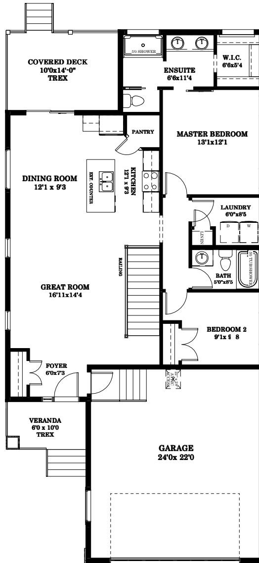
MAIN FLOOR 1246 sq. ft.
