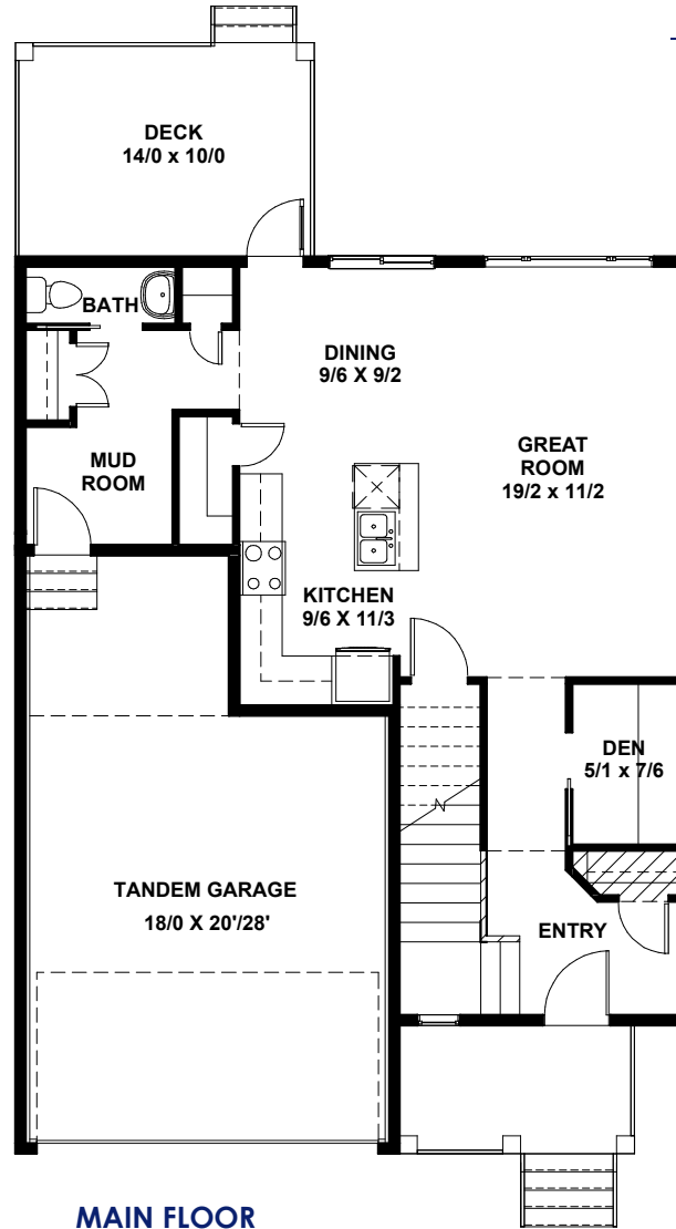
MAIN FLOOR 808 sq. ft.
