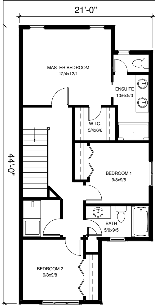
UPPER FLOOR 777 SQ.FT. 8'-1 1/8"
