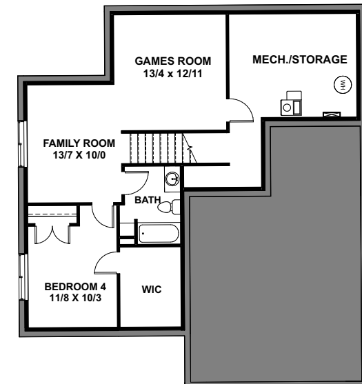
FUTURE BASEMENT 600 sq. ft.
