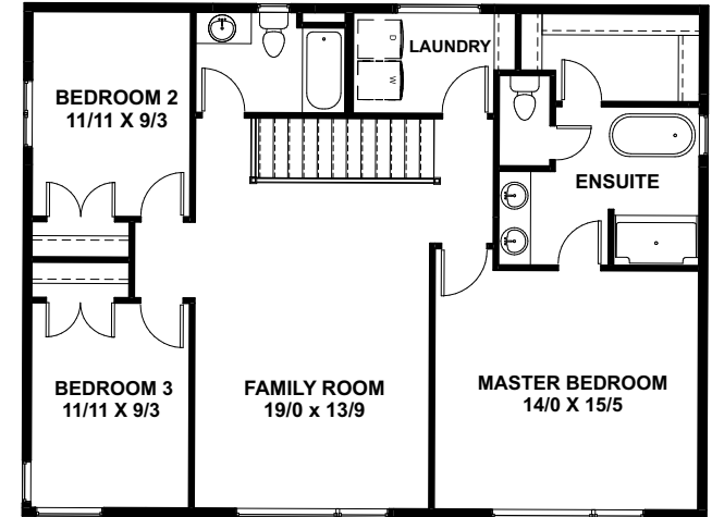
UPPER FLOOR 1200 sq. ft.
