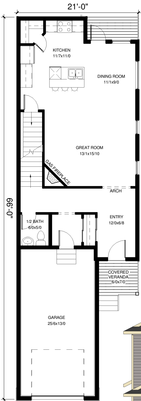
UPPER FLOOR 819 SQ. FT. 9'-1 1/8"
