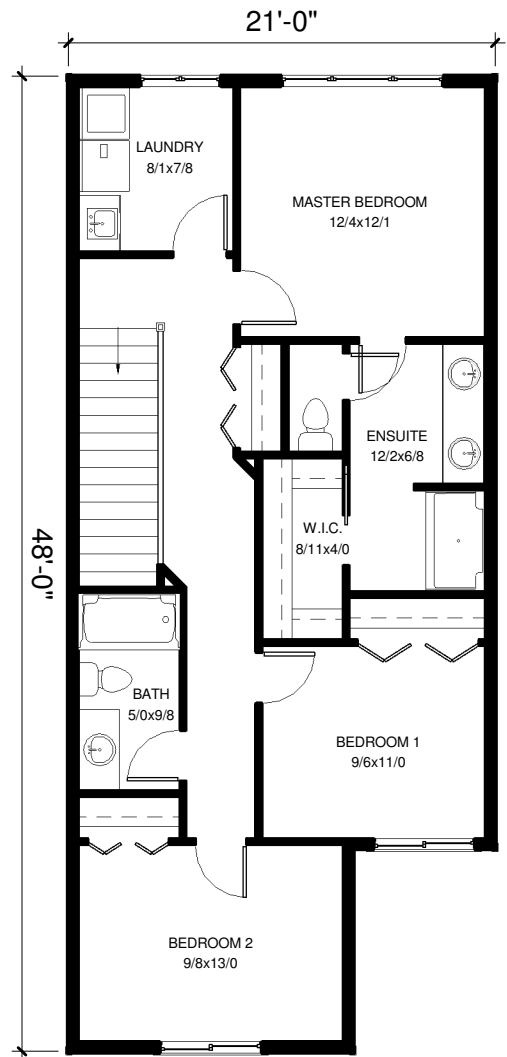
UPPER FLOOR 888 SQ. FT. 8'-1 1/8"
