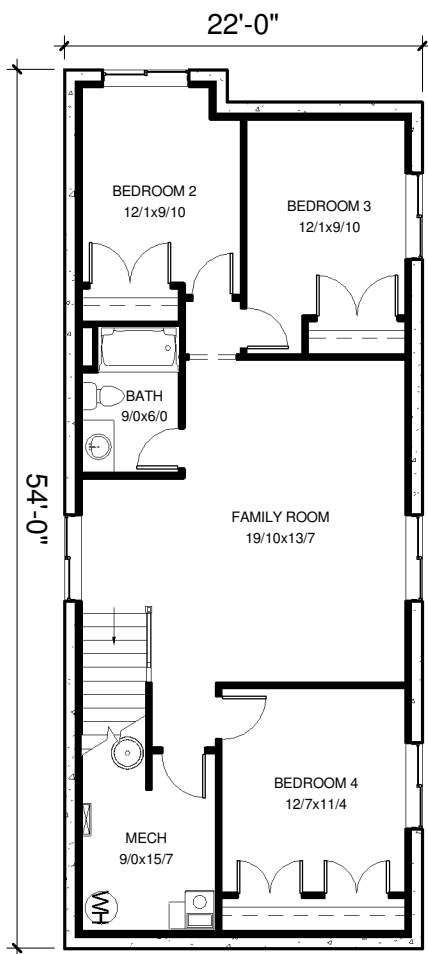
LOWER FLOOR 1029 SQ. FT. 9'-4" WALLS
